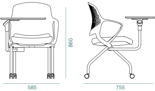
TRAINING CHAIR WITH TABLET
